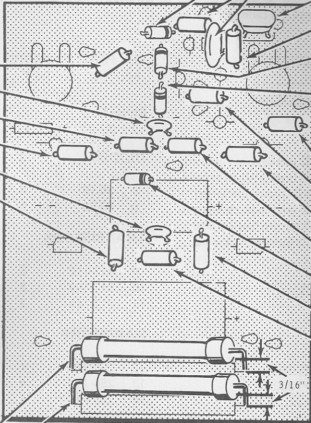
PICTORIAL 3-1
