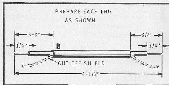
Detail 2-4C
