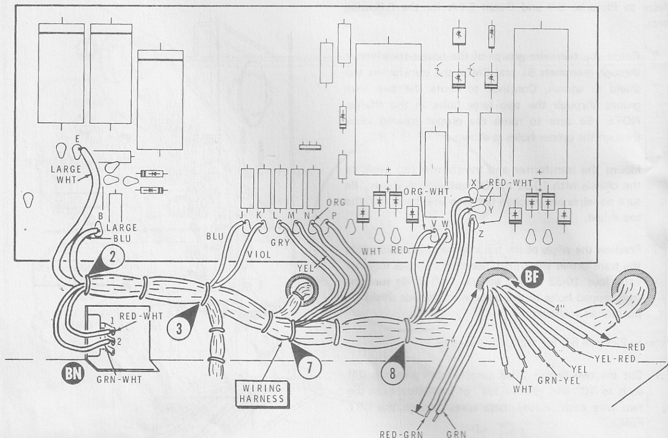
PICTORIAL 5-10
