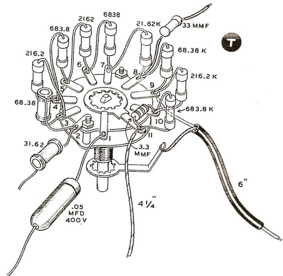
RANGE SWITCH
