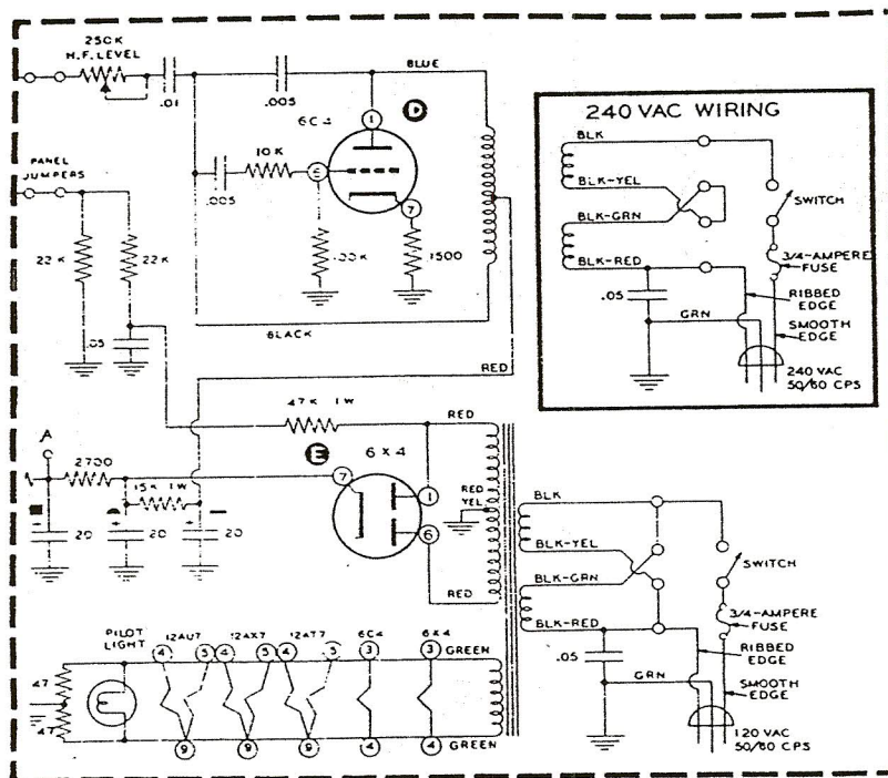
PARTIAL SCHEMATIC
