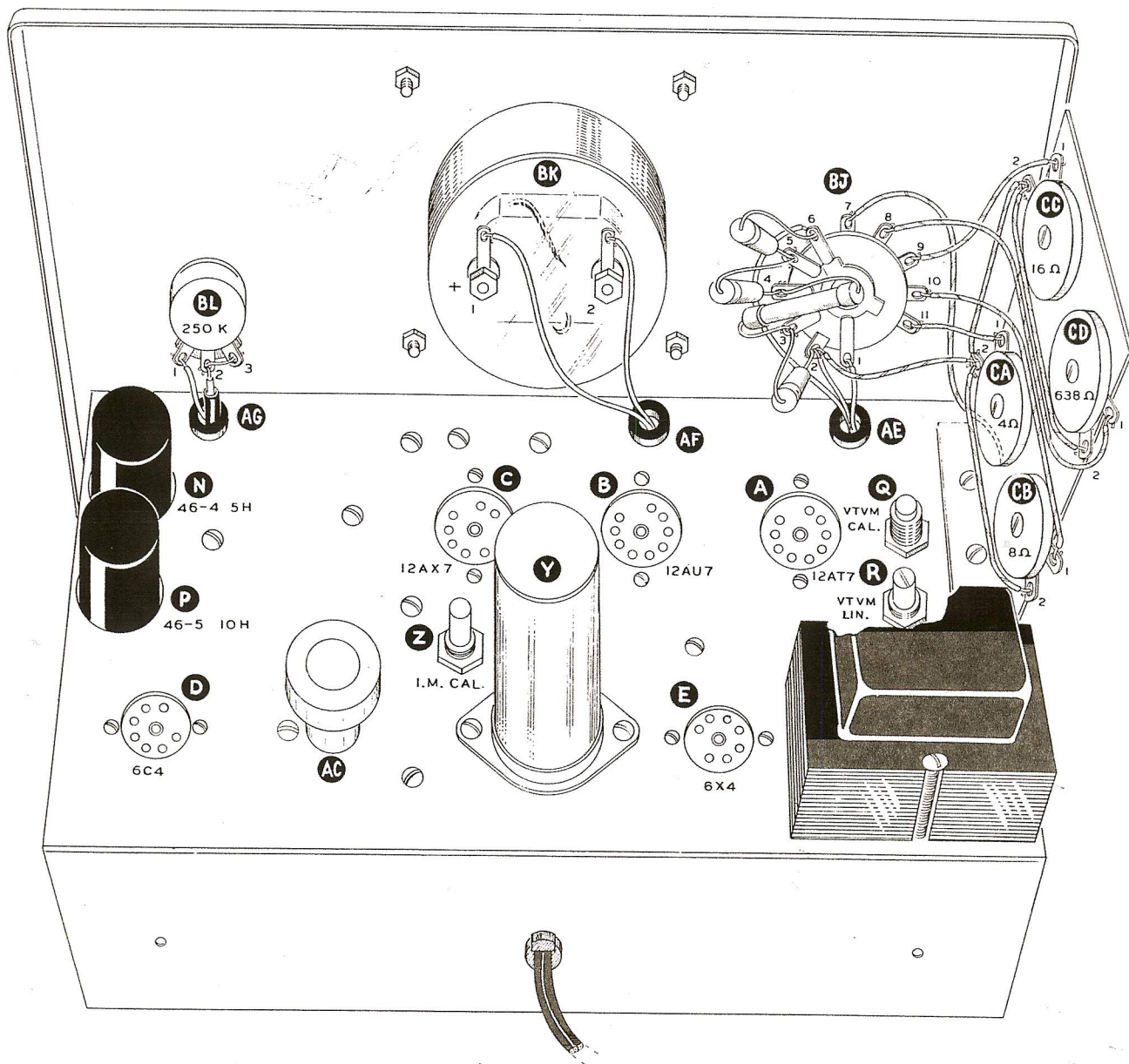
PICTORIAL 2
